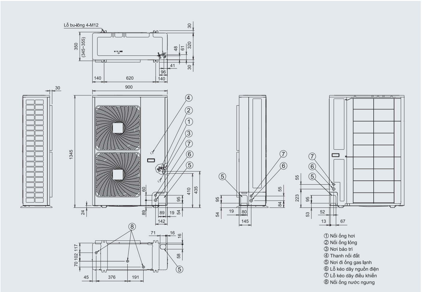
DÀN NÓNG // RNQ36MV1, RNQ36/42/48MY1
